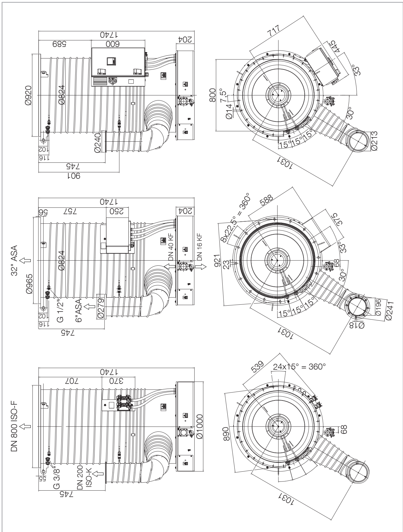
Fig. 5b Dimensional drawings for DIJ versions (DIJ 32 with junction box; DIJ 800 with plug and EEC)
