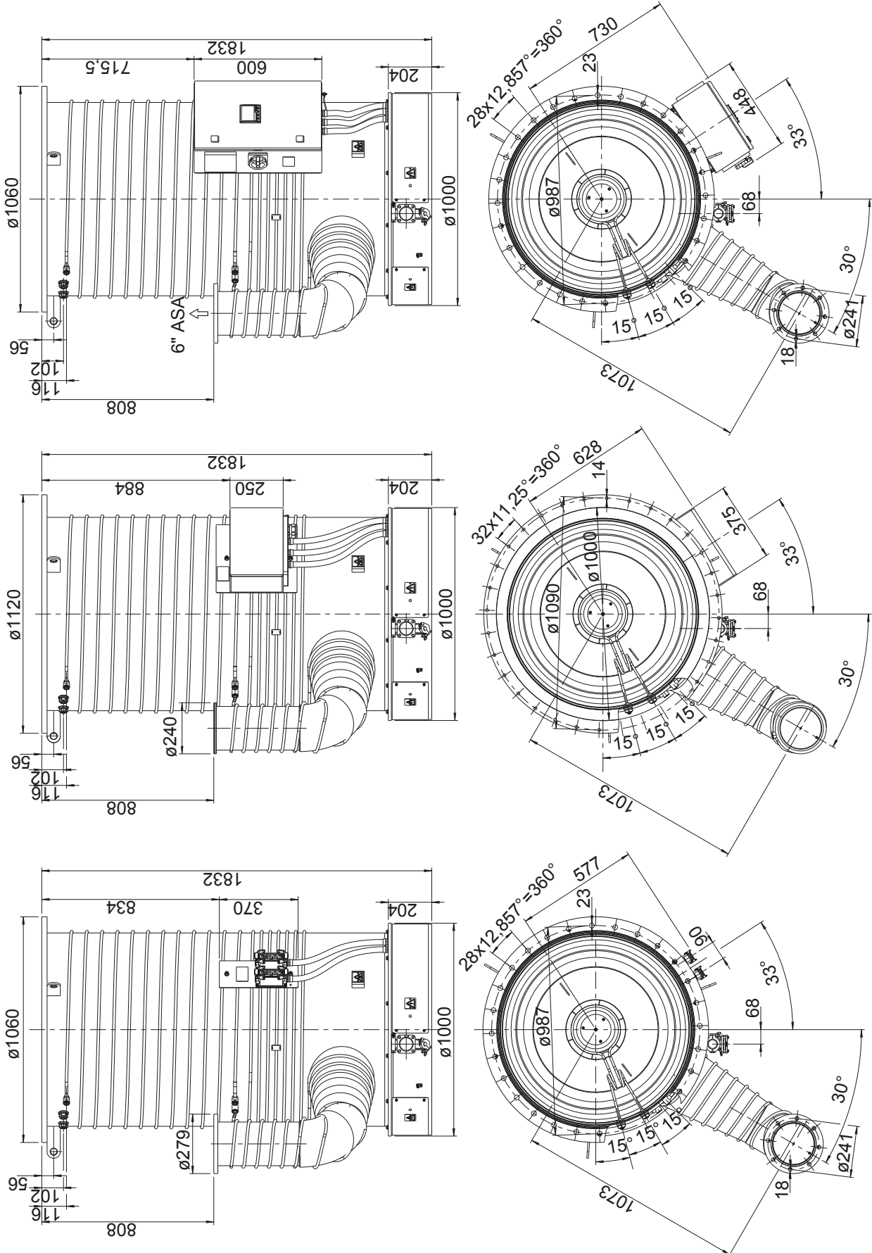
Fig. 5c Dimensional drawings for DIJ versions (DIJ 35 with plug, and EEC; DIJ 1000 with junction box)
