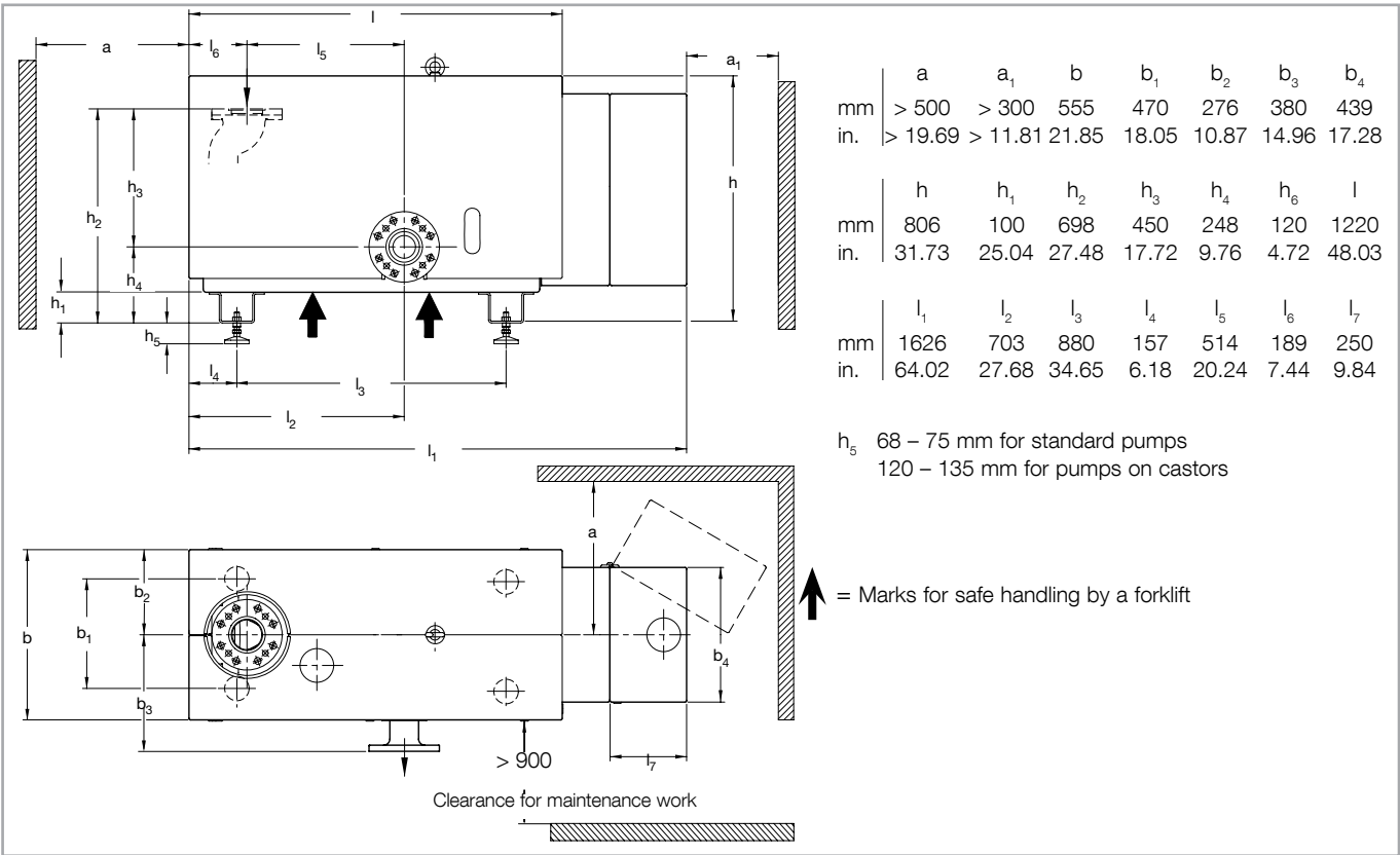
Fig. 1.6 Dimensional drawing for the SP 630
