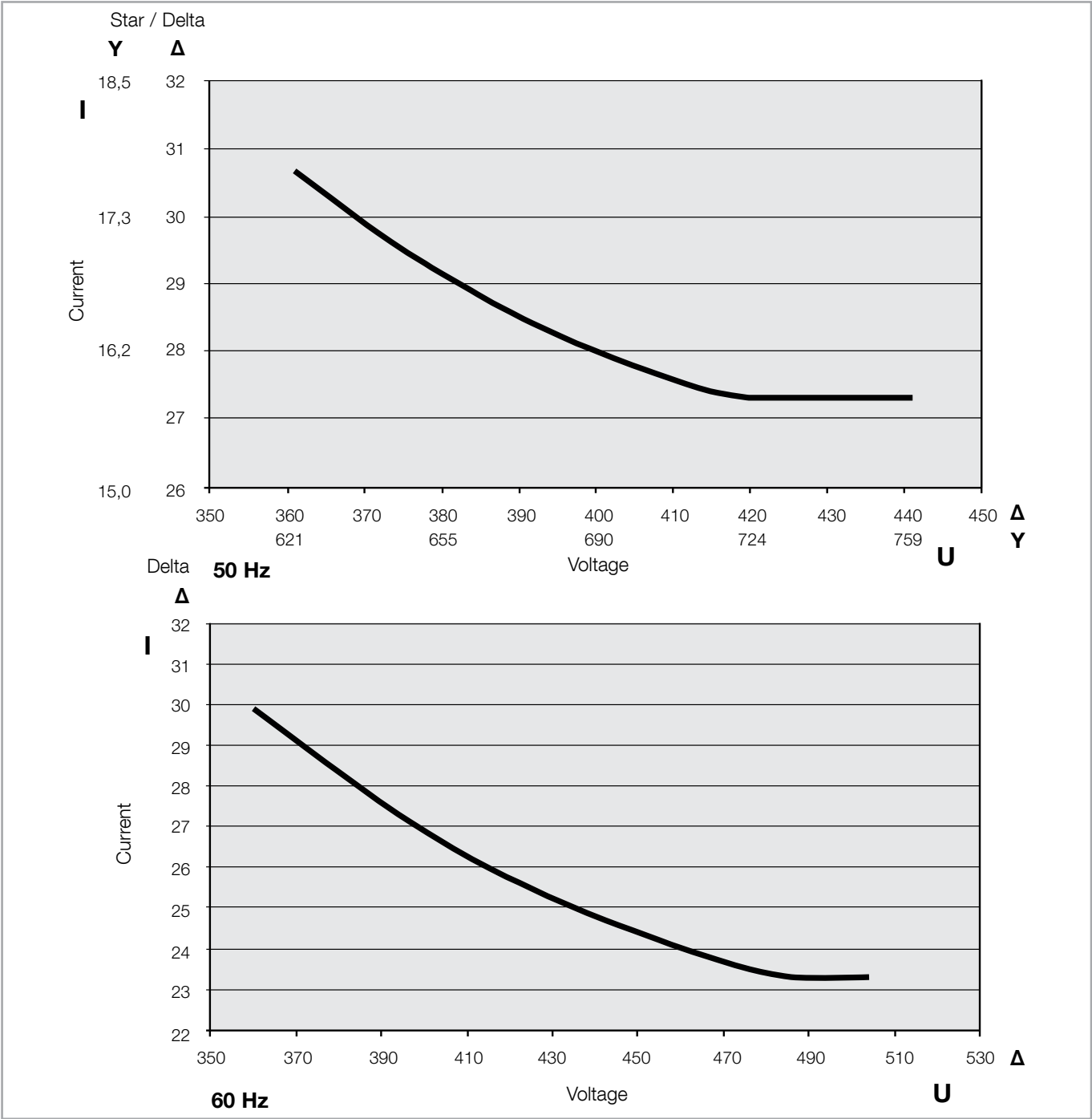
Diagram 1 Voltage/current diagram
