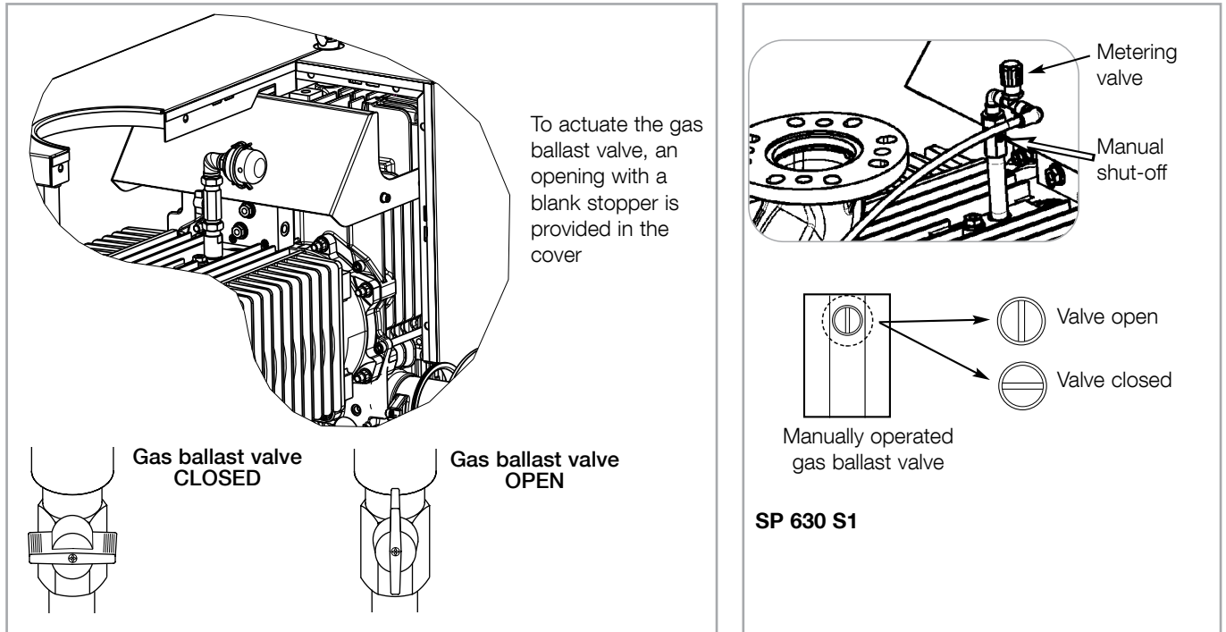
Fig. 4.4 Manually operated gas ballast valve
