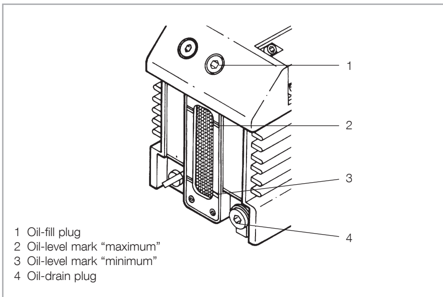
Fig. 9 Oil change
